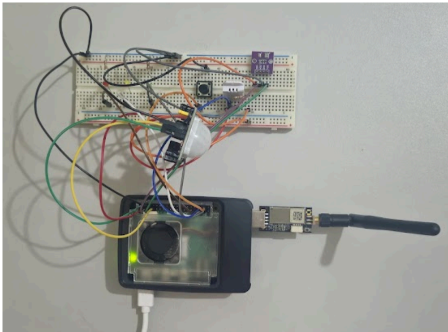
Figure 09: complete raspberry setup
