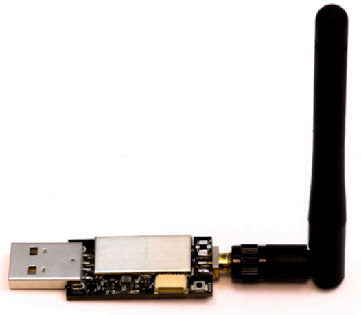
Figure 04: Crazyradio 2.0
