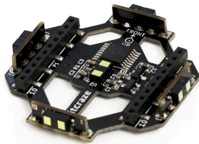
Figure 05: Multiranger Deck
