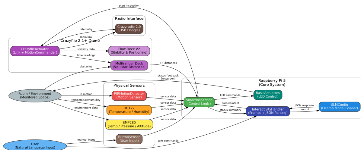
Figure 08: dataflow architecture
